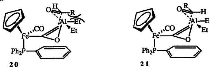
Scheme 8
