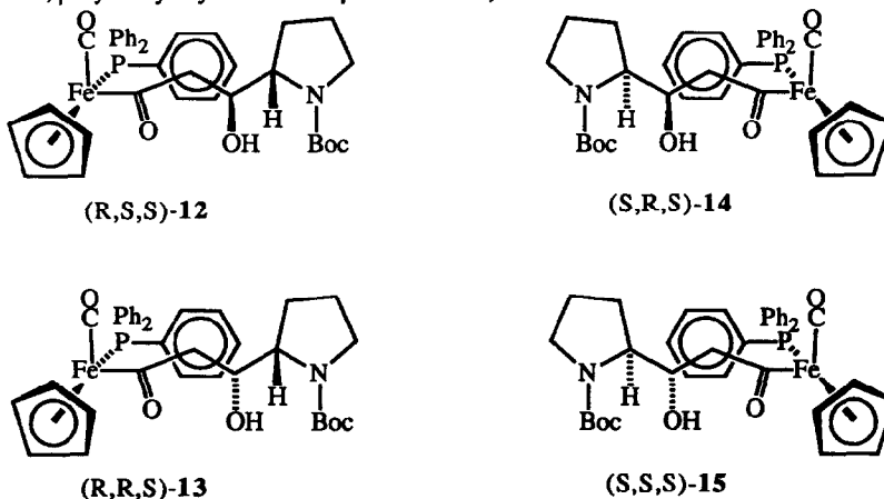
Scheme 3
