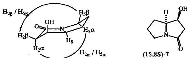
Figure 3 Long Range ^1\text{H} - ^1\text{H} n.m.r. Couplings in (1 S ,8 S )-7.
