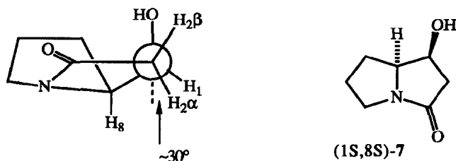
Figure 2 Newman Projection along the C2 - C1 axis in (1 S ,8 S )-7.
