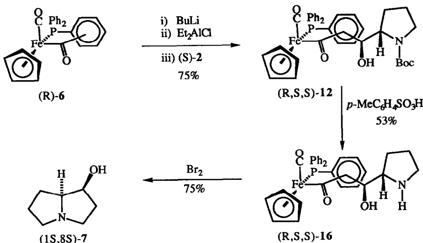
Scheme 7
